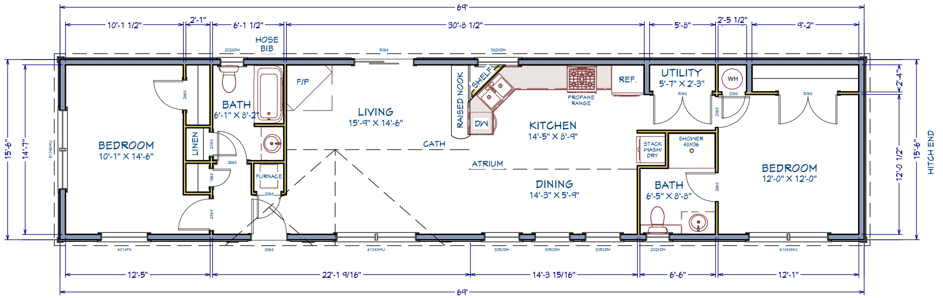
FLOOR PLAN
